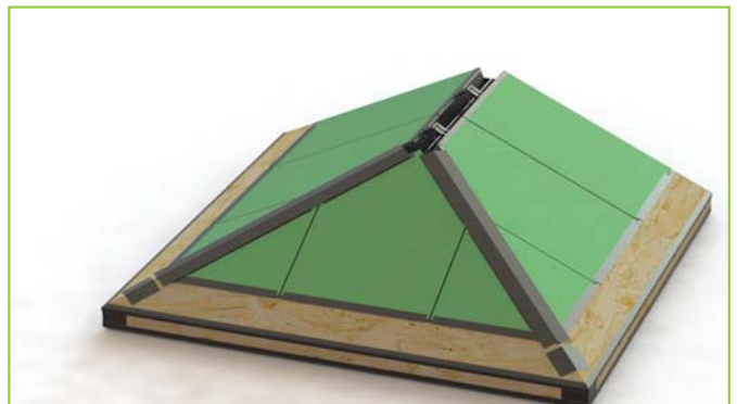
Super insulated Unideck panels (0.12 W/m 2 K U value)
