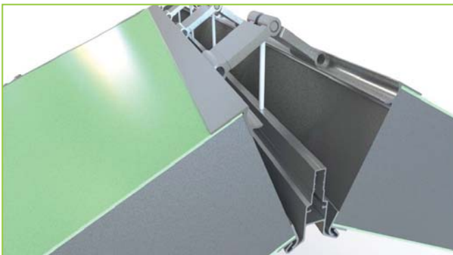
An internal aluminium framework for hips, ridge and starter bars
